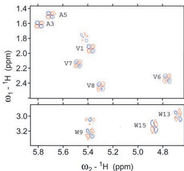
FIGURE 5 Overlay of the \text{H}\alpha\text{-H}\beta regions of two 500-MHz phase-sensitive COSY spectra of gramicidin in SDS micelles, recorded in \text{D}_2\text{O} at 30^\circ\text{C} , in the absence ( upper contour level ) and presence ( lower contour level ) of F3. For clarity, only one contour level was plotted for each spectrum; the blue and red were used to differentiate negative and positive phase of cross-peaks, respectively. The spectra were acquired as a 1360 \times 6400 data matrix with identical spectral widths in the two dimensions. Data were apodized with Gaussian windows, before zero filling to 2000 \times 9600 . The excellent overlap of COSY cross-peaks in the absence and presence of 14.8 mM F3 suggested that the F3 effects on side-chain orientations were minute.
