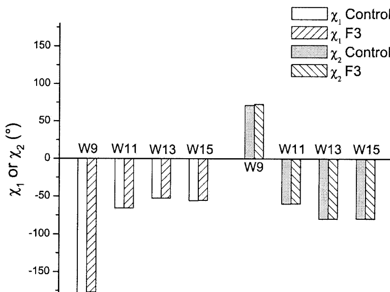
FIGURE 6 Comparison of tryptophan side chain orientations in the absence and presence of 14.8 mM F3. The dihedral angles \chi_1 ( \text{HN-C}_\alpha\text{-C}_\beta\text{-C}_\gamma ) and \chi_2 ( \text{C}_\alpha\text{-C}_\beta\text{-C}_\gamma\text{-C}_{\delta 1} ) were the averaged results from 30 refined structures.
